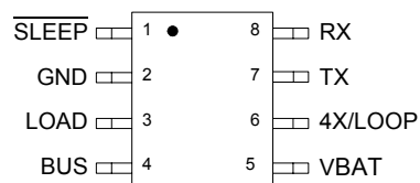
Figure 3. 33990 Pin Connections
