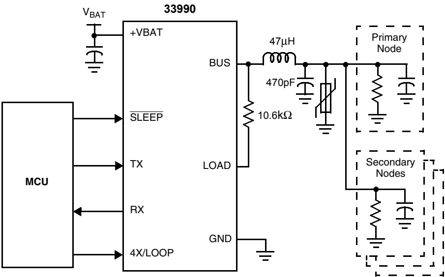
Figure 14. Typical Application
