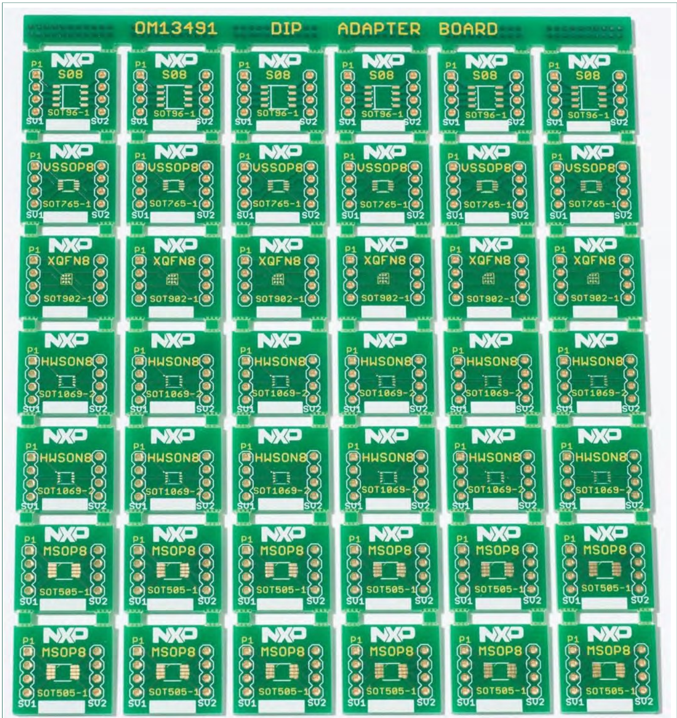
Figure 2. Panel A – consisting of six positions each of SO8, VSSOP8, XQFN8, 2xHWSON8 and 2xMSOP8
