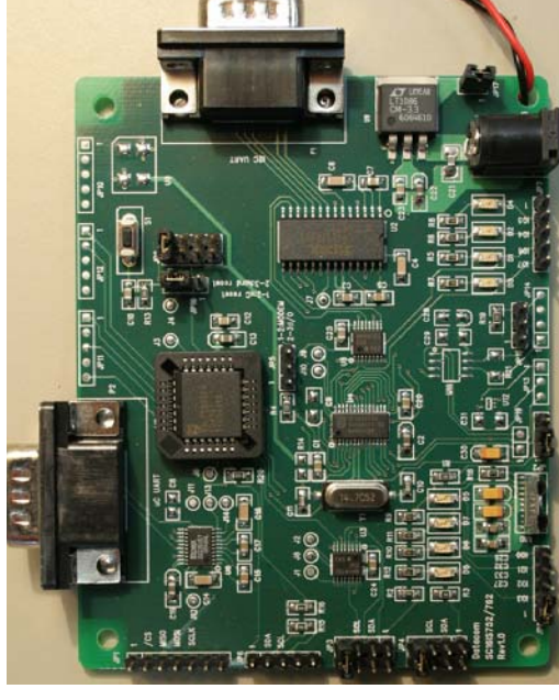
I 2 C or SPI to Dual Async incl. RS-485 Support
