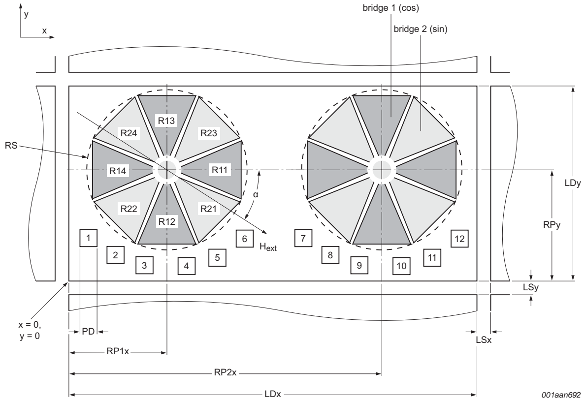
Fig 6. Bare die outline (double die)
