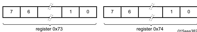
Fig 7. Data representation for CRC calculation
