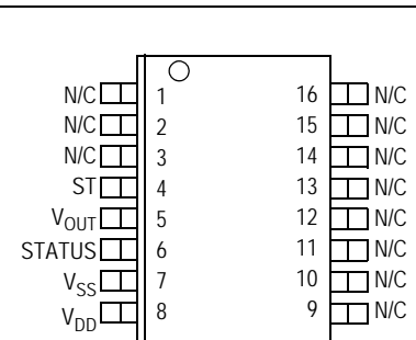
Figure 2. Pin Connections
