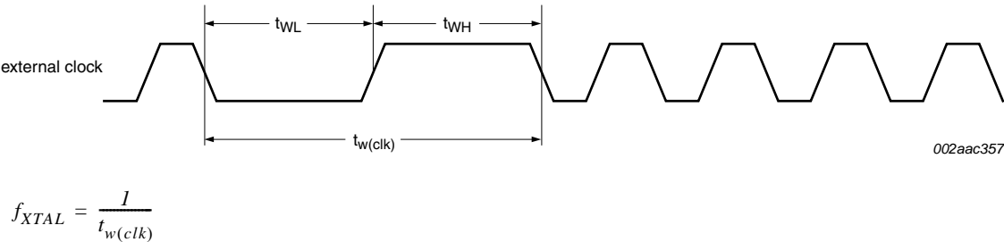
Fig 14. External clock timing
