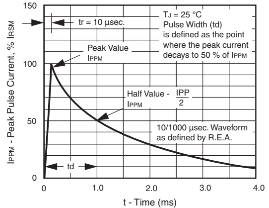
Figure 3. Pulse Waveform
