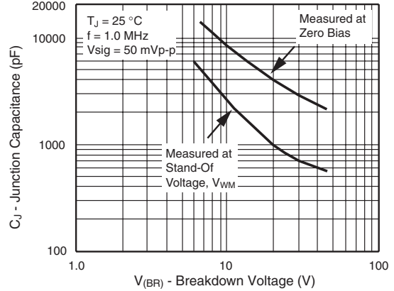
Figure 4. Typical Junction Capacitance Unidirectional
