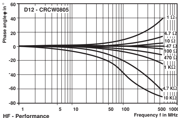
HF - Performance
