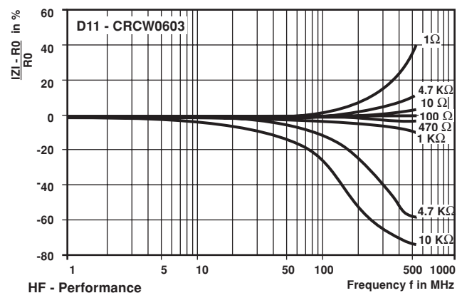
HF - Performance
