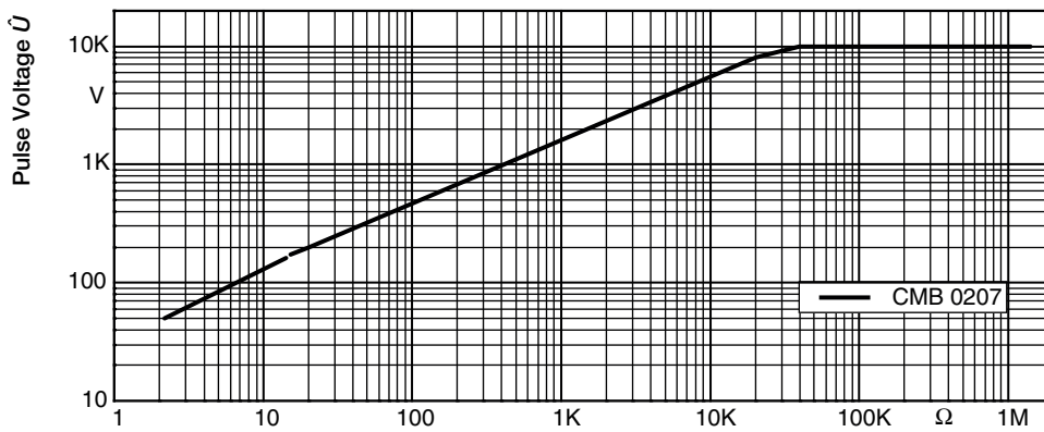
Pulse load rating in accordance with IEC 60115-1, 4.27; 10 μs/700 μs; 10 pulses at 1 min intervals; for permissible resistance change 0.5 \% \pm (0.5 \% R + 0.05 \Omega)
