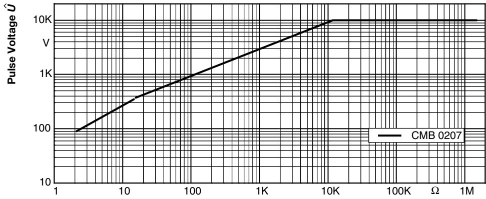
Pulse load rating in accordance with IEC 60115-1, 4.27; 1.2 μs/50 μs; 5 pulses at 12 s intervals; for permissible resistance change \pm (0.5 \% R + 0.05 \Omega)
