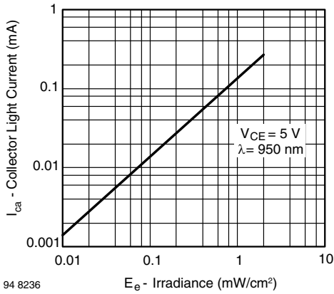
94 8236 Fig. 3 - Collector Light Current vs. Irradiance
