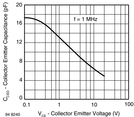
94 8240 Fig. 5 - Collector Emitter Capacitance vs. Collector Emitter Voltage
