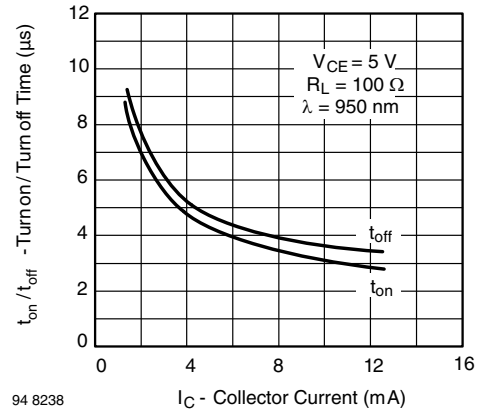
94 8238 Fig. 6 - Turn-on/Turn-off Time vs. Collector Current
