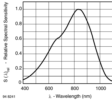
94 8241 Fig. 7 - Relative Spectral Sensitivity vs. Wavelength
