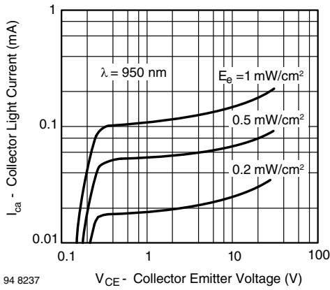
94 8237 Fig. 4 - Collector Light Current vs. Collector Emitter Voltage
