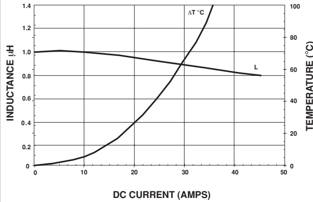
IHLP-5050CE-01 1.0 \mu H
