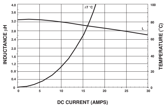
IHLP-5050CE-01 3.3 \mu H
