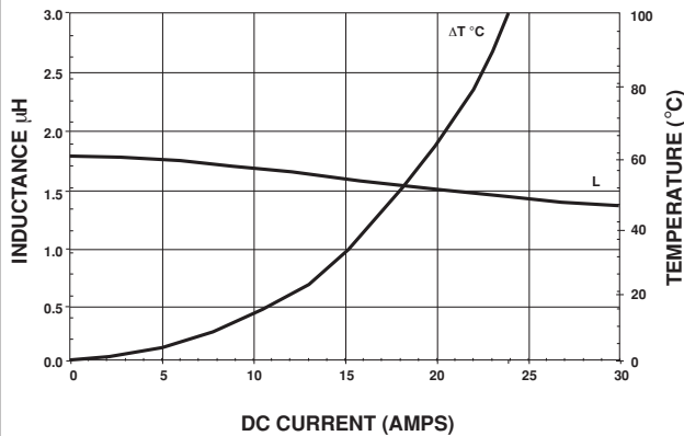
IHLP-5050CE-01 1.8 \mu H
