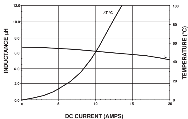
IHLP-5050CE-01 6.8 \mu H
