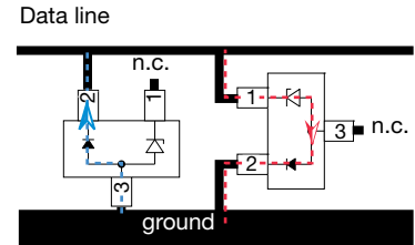
BiAs Bidirectional and Asymmetrical clamping performance for positive and negative transients.
