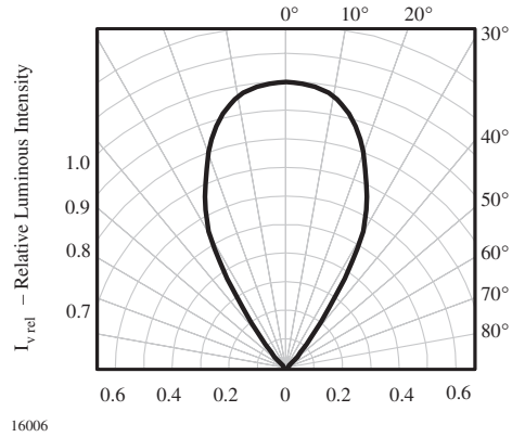
Figure 4. Rel. Luminous Intensity vs. Angular Displacement for 60^{\circ} emission angle
