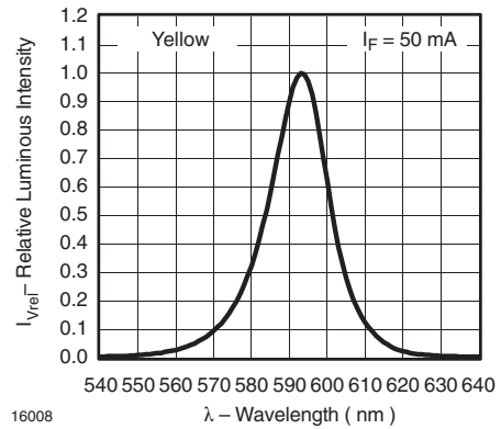
Figure 16. Relative Luminous Intensity vs. Wavelength
