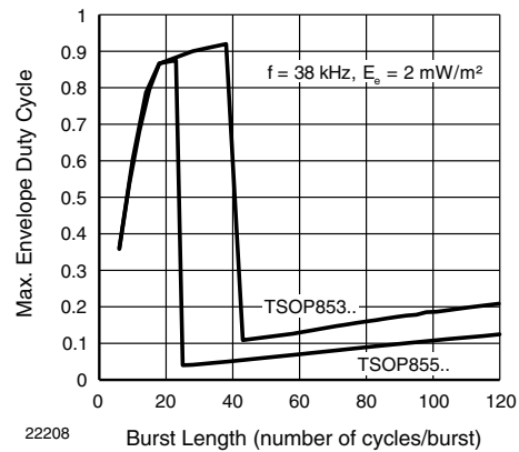
Fig. 7 - Max. Envelope Duty Cycle vs. Burst Length
