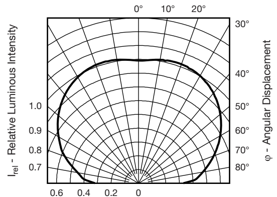
Fig. 8 - Relative Luminous Intensity vs. Angular Displacement
