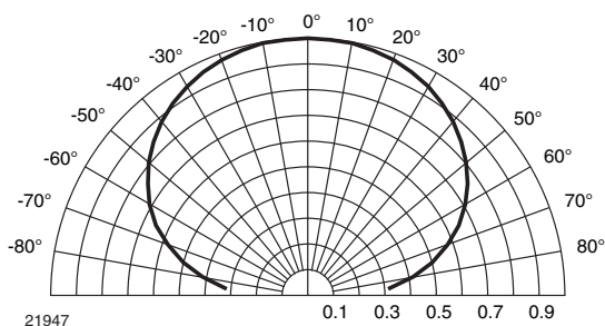
Fig. 10 - Directivity
