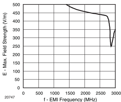
Fig. 6 - Sensitivity vs. Electric Field Disturbances
