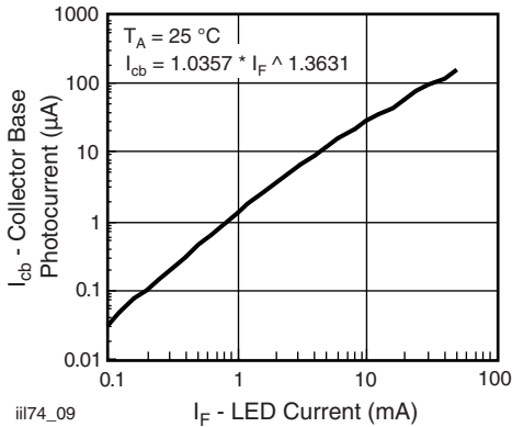
Fig. 8 - Collector Base Photocurrent vs. LED Current
