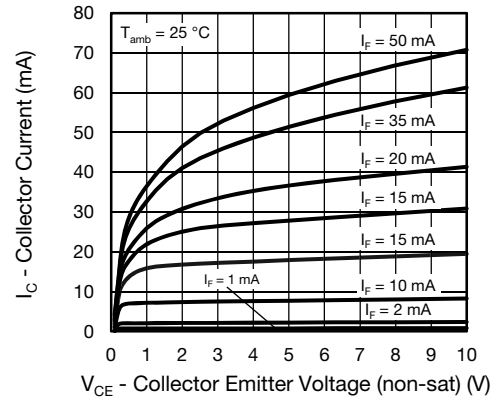
Fig. 9 - Collector Current vs. Collector Emitter Voltage (non-saturated)
