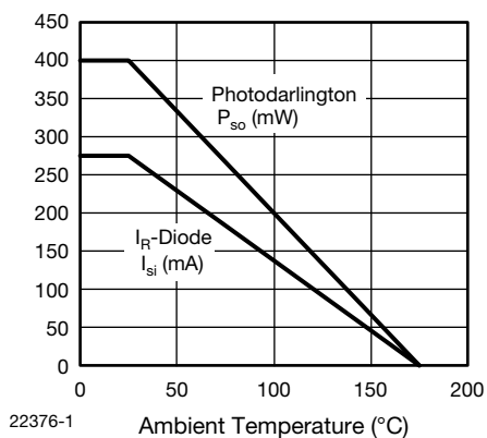
Fig. 2 - Derating Diagram
