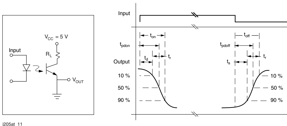
Fig. 1 - Switching Test Circuit
