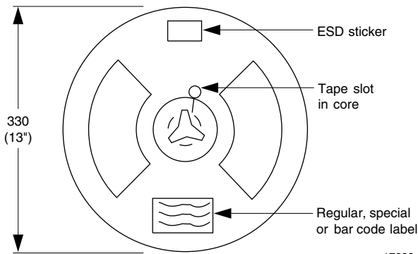
Fig. 8 - Tape and Reel Shipping Medium (EIA-481, revision A, and IEC 60286), 2000 units per reel
