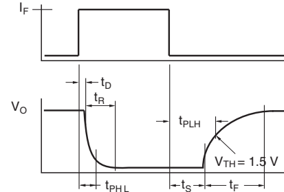
Fig. 6 - Switching Timing
