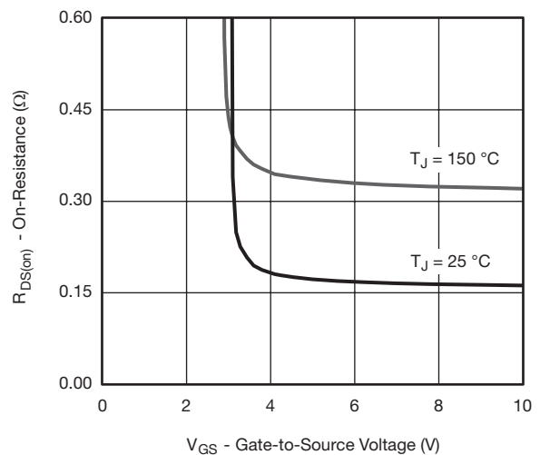
T_J = 150 °C T_J = 25 °C On-Resistance vs. Gate-to-Source Voltage
