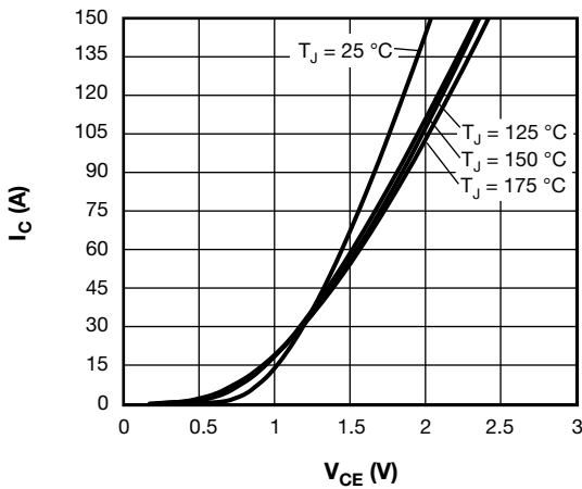
Fig. 19 - Typical Q2 - Q3 Trench IGBT Output Characteristics V_{GE} = 15\text{ V}
