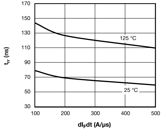
Fig. 14 - Typical D5 - D6 Clamping Diode Reverse Recovery Time vs. di_F/dt , V_{rr} = 200 V, I_F = 50 A
