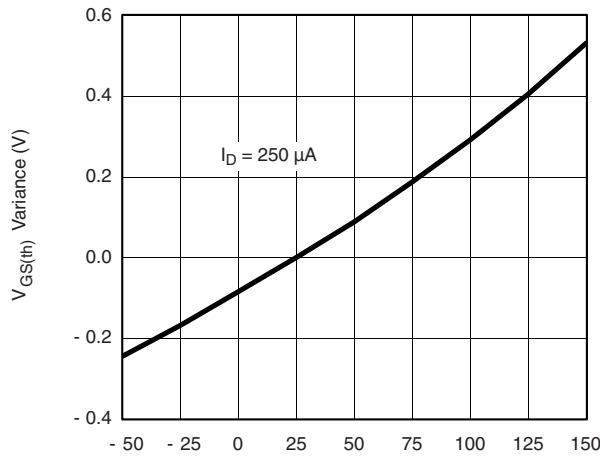
Threshold Voltage
