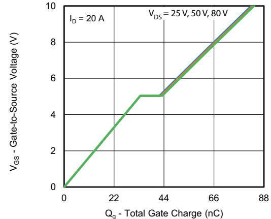
Gate Charge
