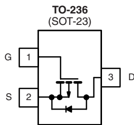
Top View Si2311DS (C1)* * Marking Code
