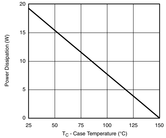
Power Derating
