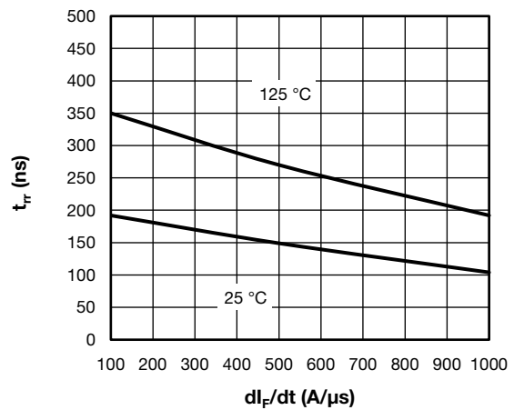
Fig. 6 - Typical Reverse Recovery Time vs. di_F/dt I_{FM} = 150 A, V_R = 300 V
