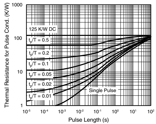
Fig. 8 - Thermal Response
