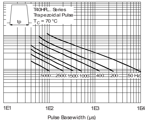
Fig. 37 - Frequency Characteristics
