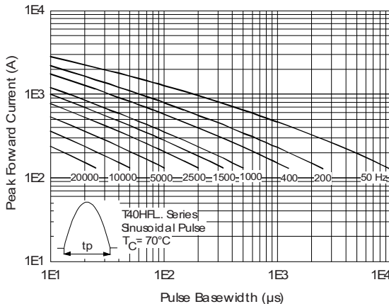
Fig. 37 - Frequency Characteristics
