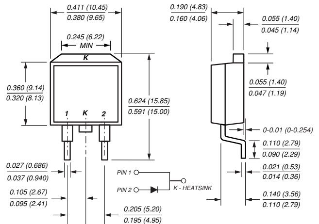
TO-263AB (MBRB16xx)
