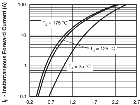
Fig. 1 - Typical Forward Voltage Drop Characteristics
