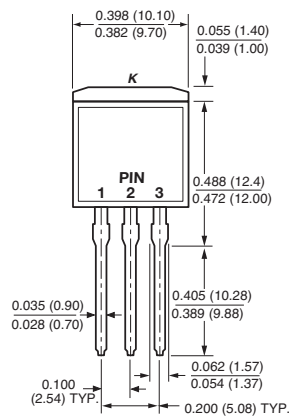
TO-262AA
