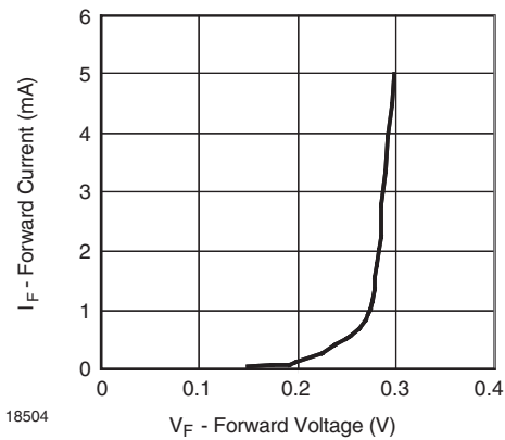
Figure 1. Typical Variation of I_F for Primary Conduction
