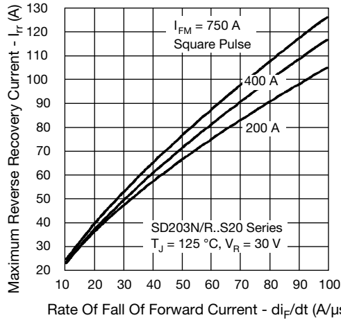
Fig. 18 - Recovery Current Characteristics
