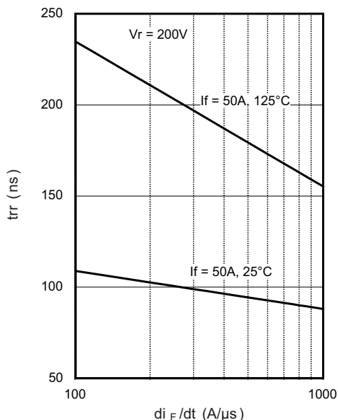
Fig. 6 - Typical Reverse Recovery Time vs. di_F/dt
