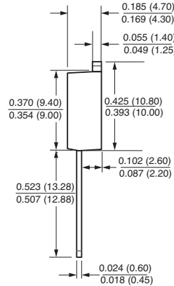
TO-262AA
