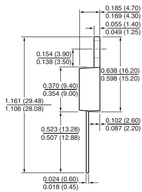
TO-220AB
