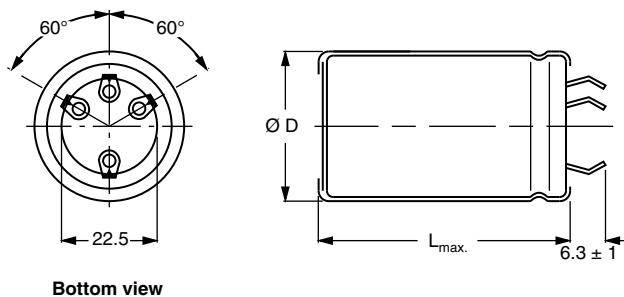
Fig. 6 - 4-Terminal snap-in
