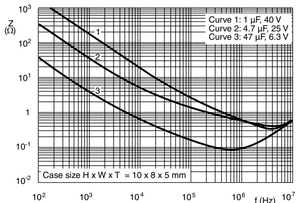
Fig. 22 - Typical impedance at 25 °C as a function of frequency
