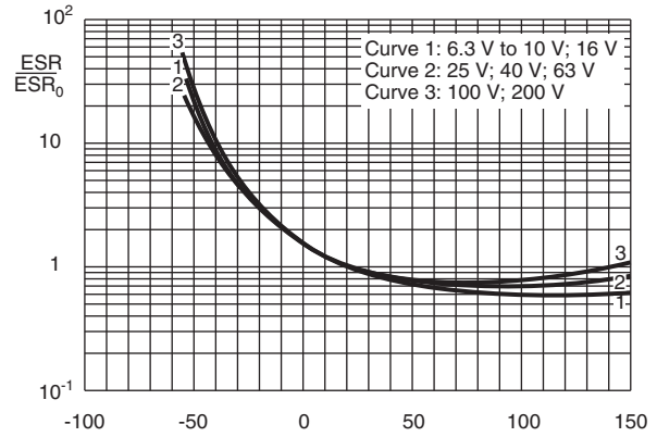
Case Ø D x L = 18 mm x 30 mm to 21 mm x 38 mm T_{amb} (°C) ESR_0 = Typical at 20 °C, 100 Hz
