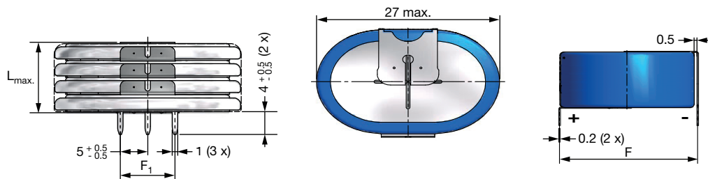
Fig. 12 - Form K: Stacked Through Hole Oval Horizontal
