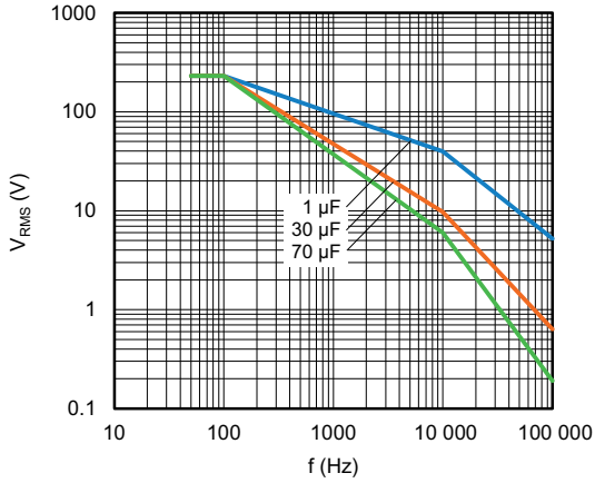
Maximum RMS voltage as function of frequency T_{amb} \leq 85^\circ C ; U_n = 230 V_{AC}
