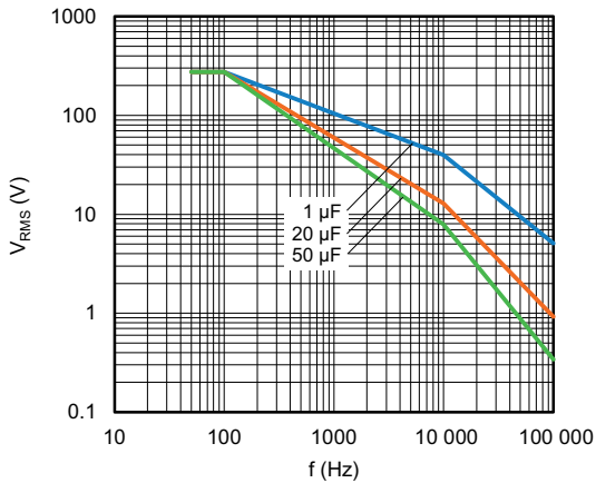
Maximum RMS voltage as function of frequency T_{amb} \leq 85^\circ C ; U_n = 275 V_{AC}
