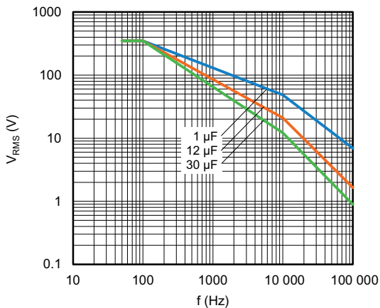
Maximum RMS voltage as function of frequency T_{amb} \leq 85^\circ C ; U_n = 350 V_{AC}
