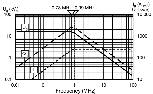
WX095220WF502##BJ1, WF095220WF502##BJ1
