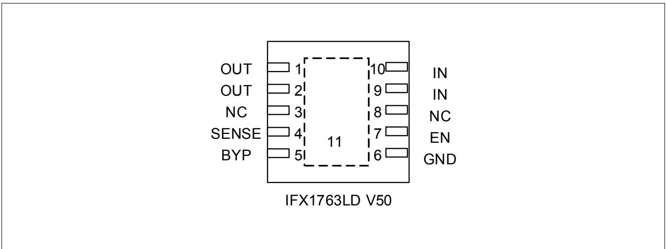
Figure 3 Pin Configuration of IFX1763LDV50 in PG-TSON10
