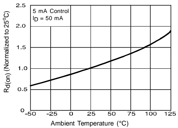
Figure 4. Typical On-Resistance
