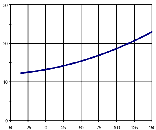
Figure 11 - R_{ds(on)} ( m\Omega ) vs T_j ( ^\circ\text{C} )
