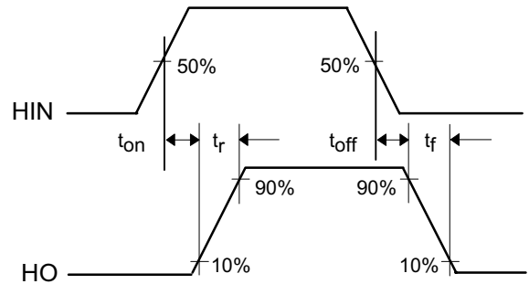
Figure 2. Switching Time Waveform Definitions
