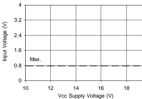
Figure 10B. Logic "0"(HIN) & Logic "1" ( \overline{\text{LIN}} ) Input Voltage vs. Voltage
