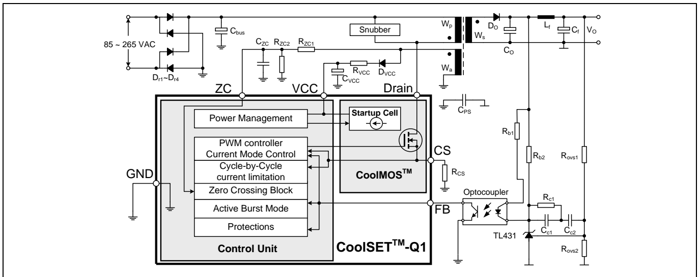
Figure 1 Typical application
